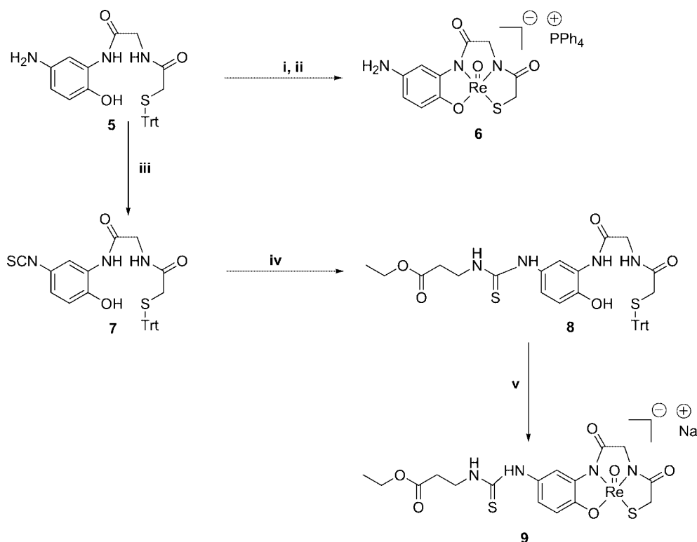
Scheme 2. Complexation and coupling studies. Reagents and conditions: (i) [\text{ReOCl}_3(\text{PPh}_3)_2] , NaOAc, 4 h, 65 °C, MeOH; (ii) \text{PPh}_4\text{Cl} , 30 min, room temp., MeOH/ \text{CH}_2\text{Cl}_2 , 58%; (iii) \text{Cl}_2\text{CS} , 1 h, room temp., THF, 87%; (iv) \beta -alanine ethyl ester hydrochloride, \text{NEt}_3 , 3 h, room temp., THF, 91%; (v) [\text{ReOCl}_3(\text{PPh}_3)_2] , NaOAc, 4 h, 65 °C, MeOH, 60%.
