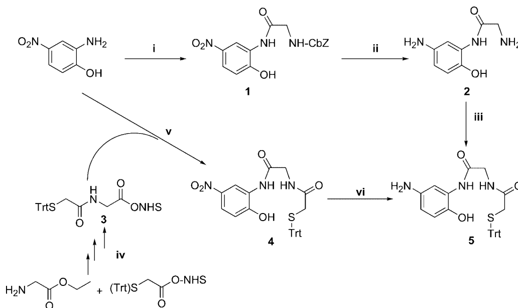
Scheme 1. Synthesis of ligand 5 . Reagents and conditions: (i) N -CbZ-glycine, DCC, THF, 44%; (ii) H 2 , Pd/C, MeOH, 95%; (iii) (Trt)SCH 2 COONHS, Et 3 N, 5 h, 40 °C, ACN, 55%; (iv) ref. [14d] , 64%; (v) 3 , DMAP, 4 h, 60 °C, ACN, 92%; (vi) Raney nickel, NH 2 NH 2 ·H 2 O, 1,2-dichloroethane/EtOH, 78%.
